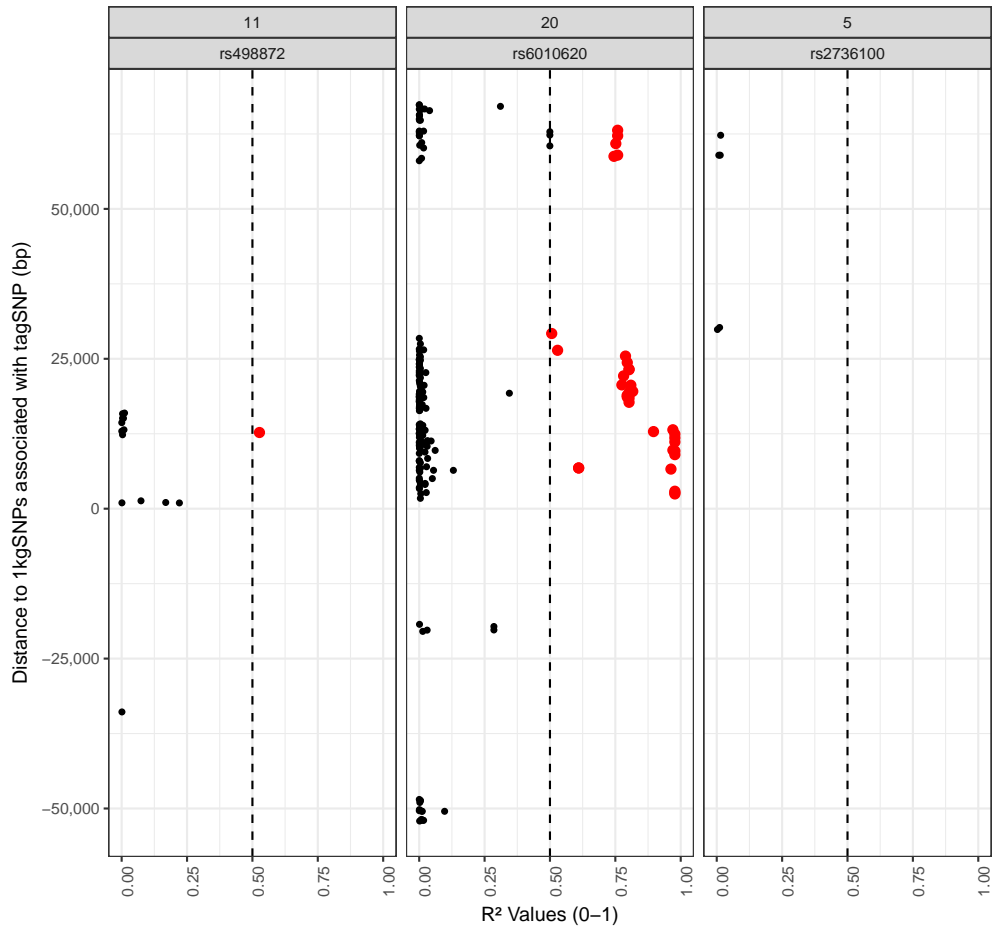
Figure 4: Scatter plot showing the relationship between Rsquare and Distance to tagSNP for each getFSNPs
