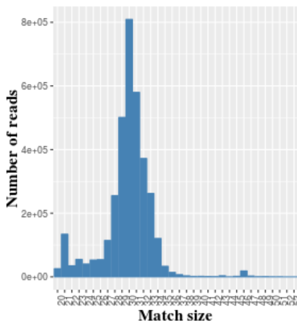
Figure 5: Histogram of read match length for example data: ctrlGAlignments .
