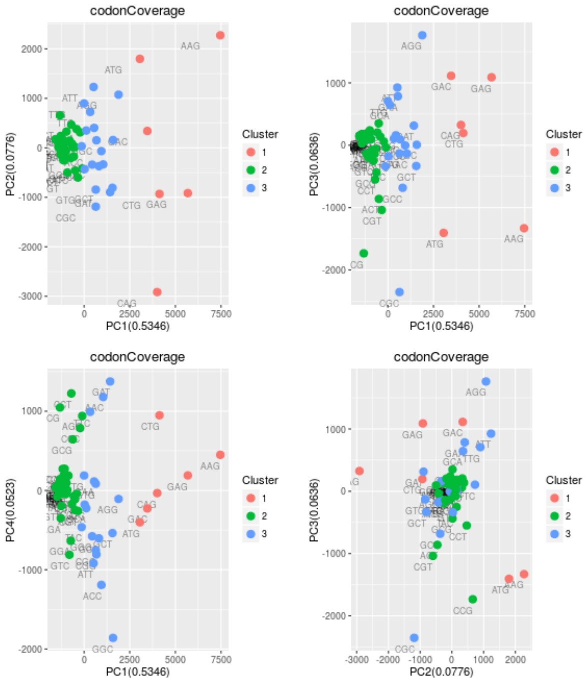
Figure 8: PCA on codon coverage for the ctrlGAlignments example data.
