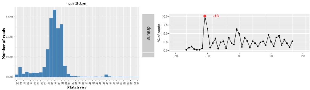
Figure 2: Histogram of read match size and read start offset to ribosome P-site for nutlin2h.bam dataset.
