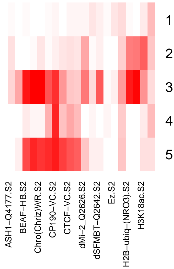
Figure 13: \text{chroGPS}^{\text{genes}} profile heatmap of the 9 unmerged clusters presented at Figure 11 after unsupervised merging of overlapping clusters (showing 20 first factors for visualization purposes). Merged clusters get concatenated names from the original clusters.
