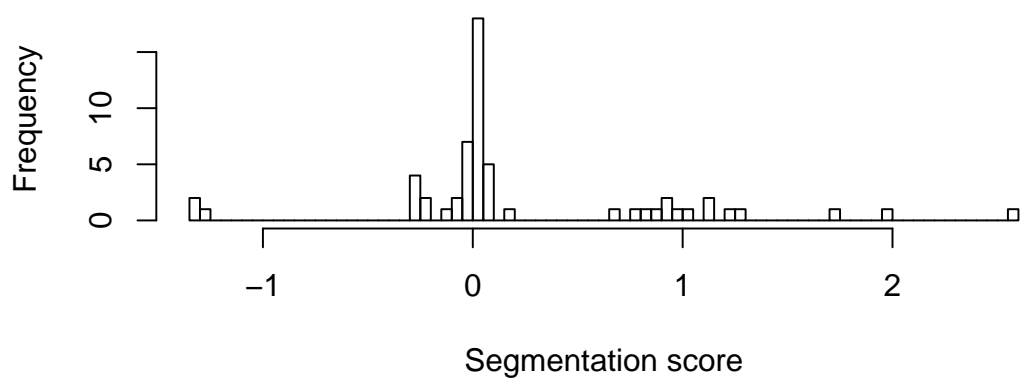
Figure 2: FCGR3B CN groups.
