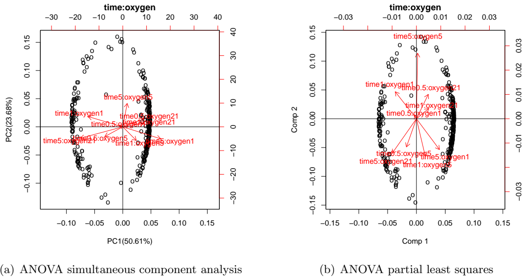
Figure 2: Biplot on the decomposed interaction coefficients ( time \times oxygen ) on genes satisfying the F test with p value < 0.001 . Notice that the interaction matrix in the ASCA model is of rank 9. Thus, 9 arrows are expected and the score of the 305 selected subjects are projected onto the space spanned by the first two principal components in Figure 2(a).
